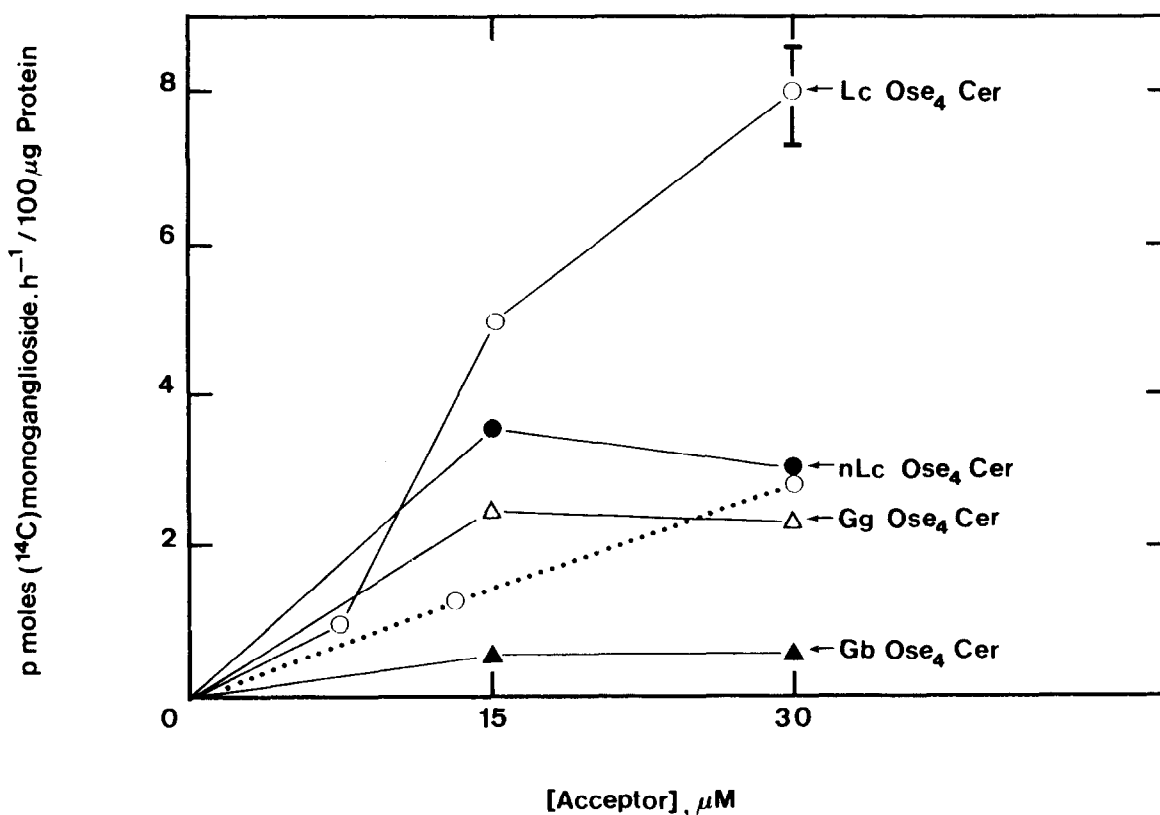
Fig.1. Incorporation of ^{14} C from CMP-[ ^{14} C]sialic into monosialoganglioside fractions as a function of glycolipid acceptor concentration. (○---○) Galactose oxidase treated LcOse 4 Cer [4].
